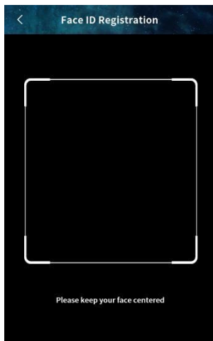
Face registration
