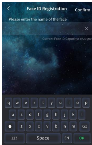
Face registration
